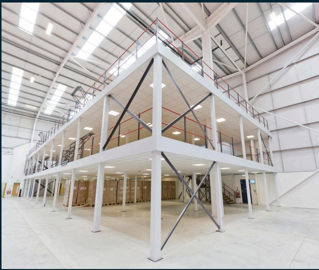
MEZZANINE FLOOR
